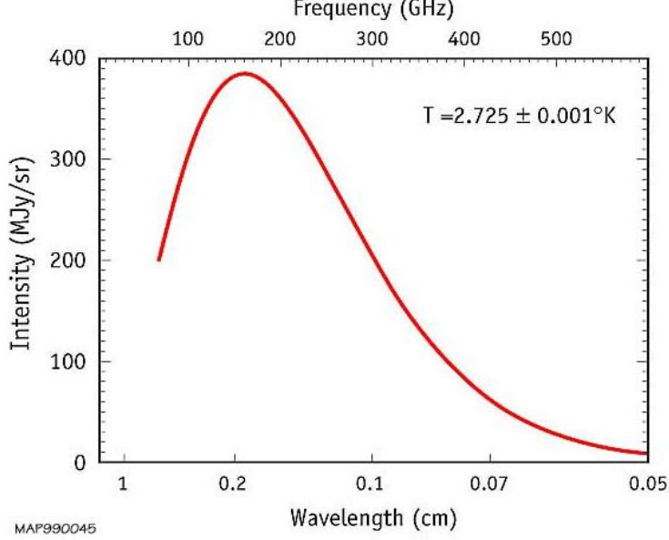
Figure 7. The FIRAS measurement of the thermal distribution of the cosmic microwave background photons. The experimental points lie on the theoretical red curve, with errors that are smaller than the width of the curve. (Figure credit: https://map.gsfc.nasa.gov/universe/bb_tests_cmb.html .)
